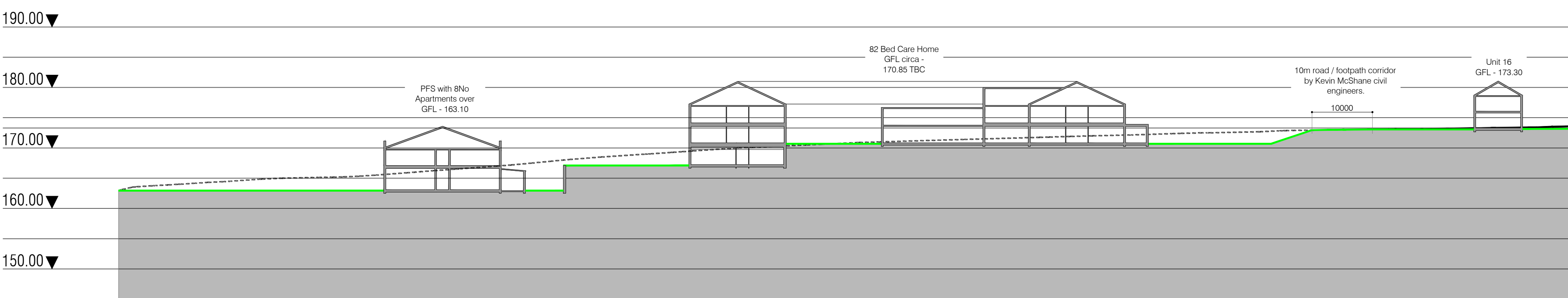
Proposed site section A-A scale 1:500
